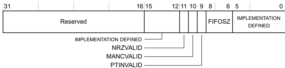
Figure C1-27 TPIU_TYPE register bit assignments
