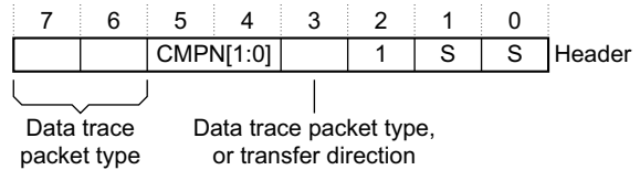
Figure D-18 Data trace packet header format
