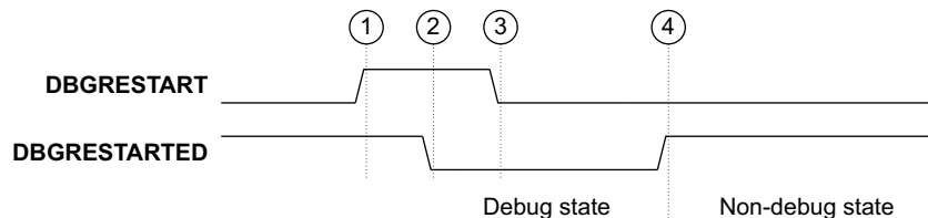
Figure C1-1 Handshake between DBGRESTART and DBGRESTARTED
