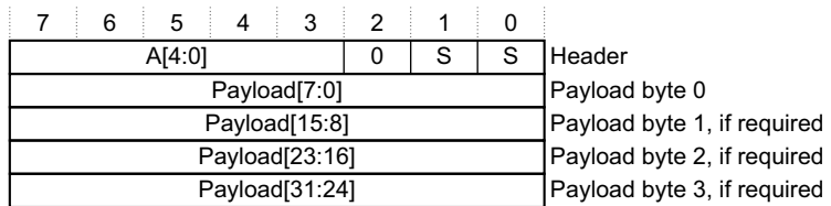
Figure D-11 Instrumentation packet format
