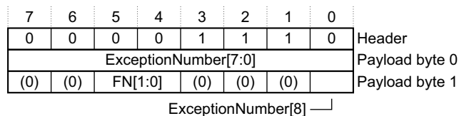
Figure D-15 Exception trace packet format
