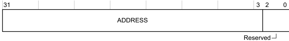
Figure B3-20 FPCAR bit assignments
