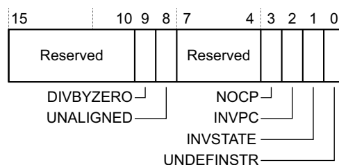
Figure B3-14 UFSR bit assignments
