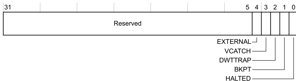
Figure C1-2 DFSR bit assignments
