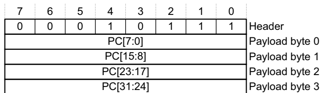
Figure D-16 Periodic PC sample packet format
