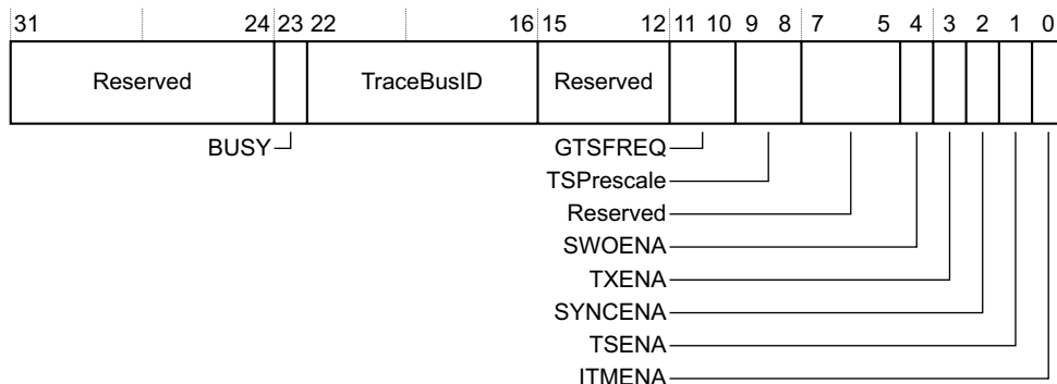
Figure C1-11 ITM_TCR bit assignments
