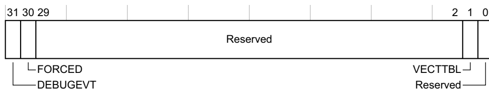
Figure B3-15 HFSR bit assignments
