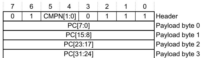
Figure D-19 Data trace PC value packet format, IDs 8, 10, 12, or 14
