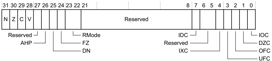
Figure A2-2 FPSCR bit assignments
