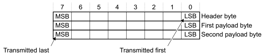
Figure D-1 Convention for packet descriptions
