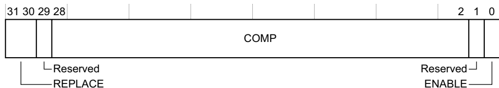
Figure C1-30 FP_COMP n register bit assignments
