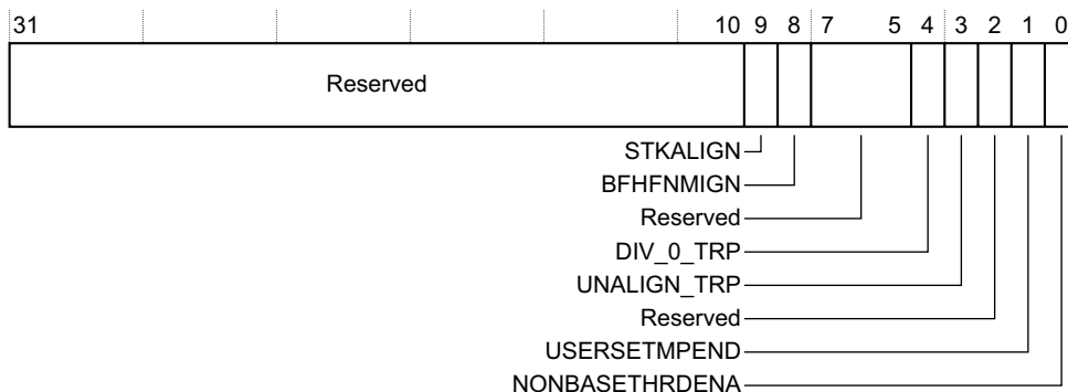
Figure B3-6 CCR bit assignments
