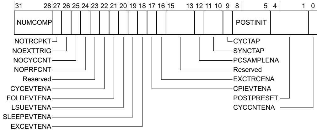
Figure C1-12 DWT_CTRL register bit assignments
