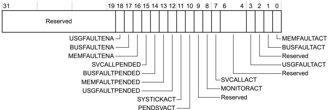
Figure B3-10 SHCSR bit assignments
