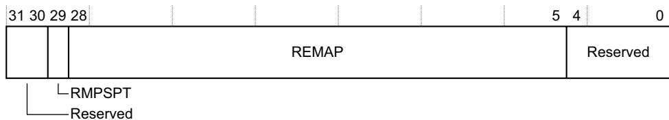
Figure C1-29 FP_REMAP register bit assignments
