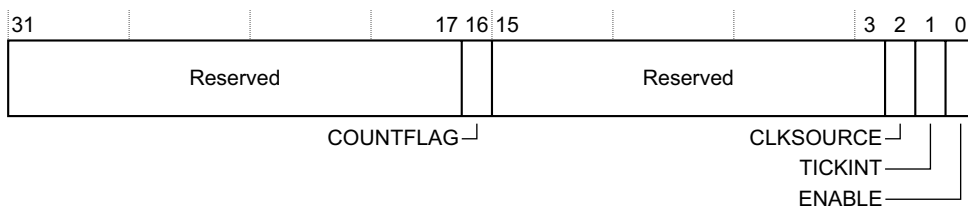
Figure B3-24 SYST_CSR bit assignments
