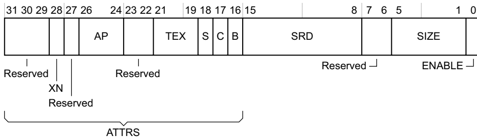
Figure B3-38 MPU_RASR bit assignments
