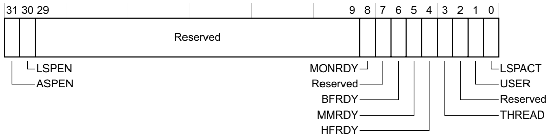
Figure B3-19 FPCCR bit assignments
