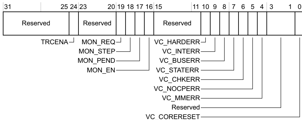
Figure C1-6 DEMCR bit assignments
