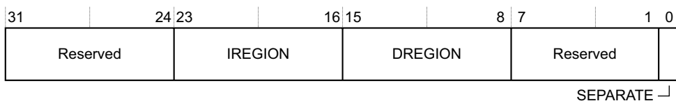
Figure B3-34 MPU_TYPE register bit assignments
