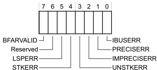
Figure B3-13 BFSR bit assignments
