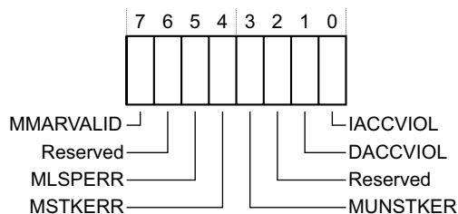
Figure B3-12 MMFSR bit assignments
