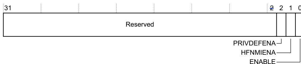
Figure B3-35 MPU_CTRL Register bit assignments
