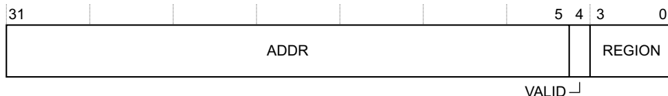
Figure B3-37 MPU_RBAR bit assignments
