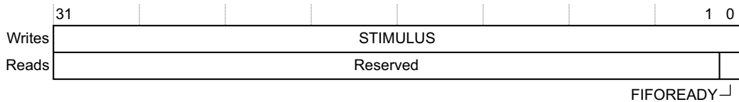
Figure C1-8 ITM_STIM x register bit assignments
