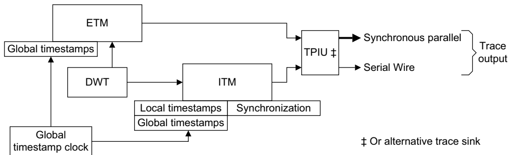
Figure C1-7 Relationship between ITM and other debug components
