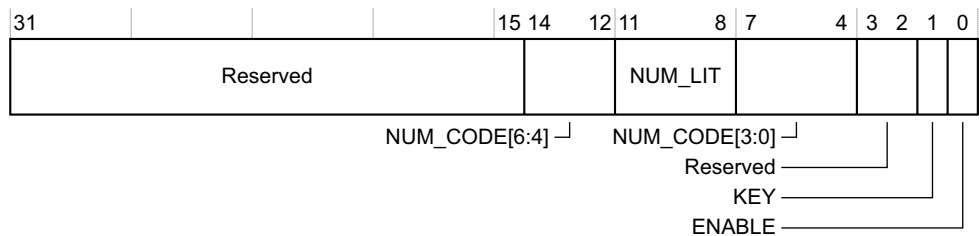
Figure C1-28 FP_CTRL register bit assignments
