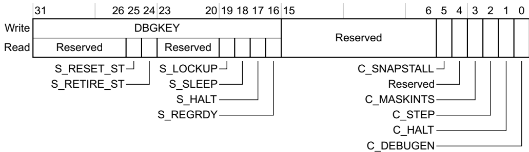
Figure C1-3 DHCSR bit assignments
