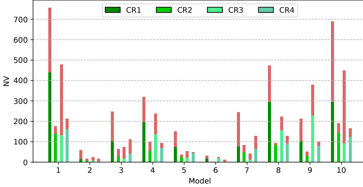
Fig. 7. Fixing Results for Each Model
