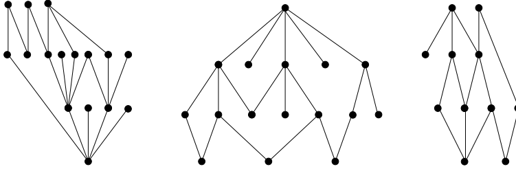
Figure 3: Three composite dags that our expanded framework can schedule optimally; all edges represent arcs that point upward. Only the middle of these dags could be scheduled optimally using the framework of [16].
