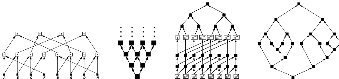
Figure 2: Data-dependency dags for four computations: matrix multiplication, a wavefront computation, the discrete Laplace transform, a divide-and-conquer computation.
