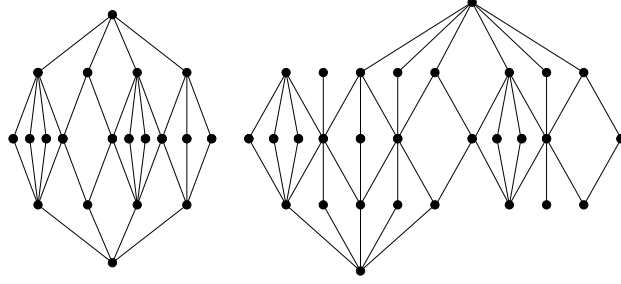
Figure 6: Two dags that can now be scheduled IC optimally. Edges represent arcs that point upward.
