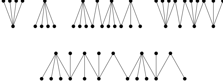
Figure 4: Top: \mathcal{W}[4] , \mathcal{M}[4] , \mathcal{M}[4, 2, 4, 3] , \mathcal{W}[4, 2, 4, 3] ; bottom: \mathcal{P} \left[ \frac{1}{4}, 3, \frac{1}{3}, 3, \frac{1}{2}, 2, \frac{1}{4}, 3, \frac{1}{2} \right] . Edges represent arcs that point upward.
