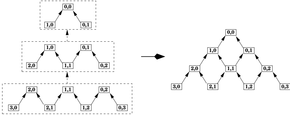
Figure 5: The reductive mesh of Fig. 2 is composite of type \mathcal{M}[2, 2, 2] \uparrow \mathcal{M}[2, 2] \uparrow \mathcal{M}[2] .
