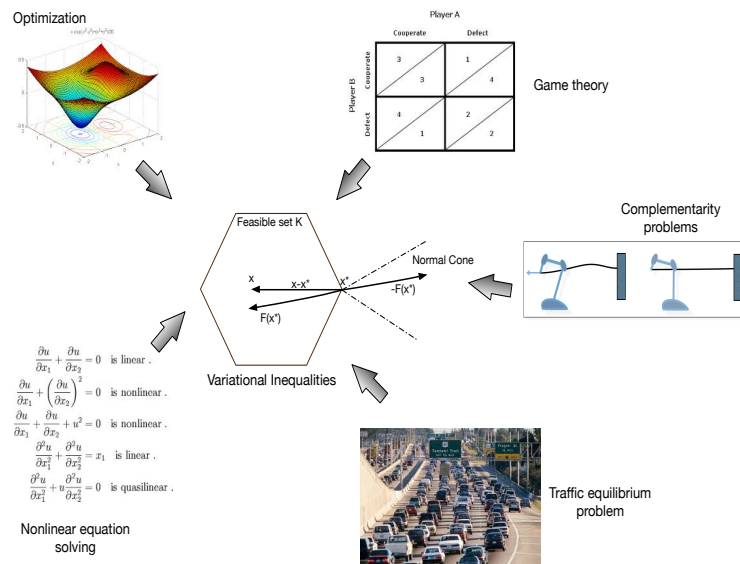
Fig. 7.1: A variety of real-world problems can be modeled as solving variational inequalities.
