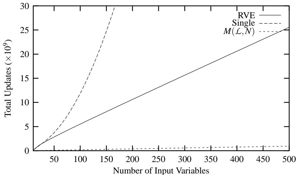
Figure 1: Plot of the expected cost of running RVE ( I_{sum}(N, r = 10) ) along with the cost of removing inputs individually, and the estimated number of updates M(\mathcal{L}, N) .
