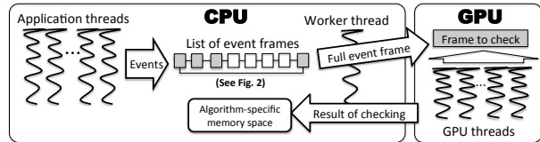
Figure 1. Components of our runtime monitoring system.
