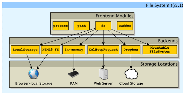
Figure 2. An overview of the DOPPIO file system. Much like an actual operating system, DOPPIO’s architecture decouples the frontend interface that programs interact with from the backend implementation that is responsible for interfacing with a particular type of persistent storage.
