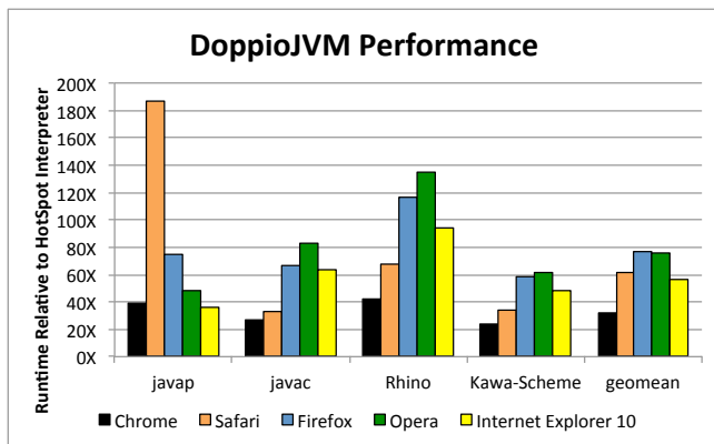
Figure 3. DOPPIOJVM’s performance on our benchmark applications relative to the HotSpot JVM interpreter bundled with Java 6. DOPPIOJVM runs between 24× and 42× slower (geometric mean: 32×) than the HotSpot interpreter in Google Chrome. Note that javap’s poor performance in Safari is due to a browser bug; we discuss this further in Section 7.
