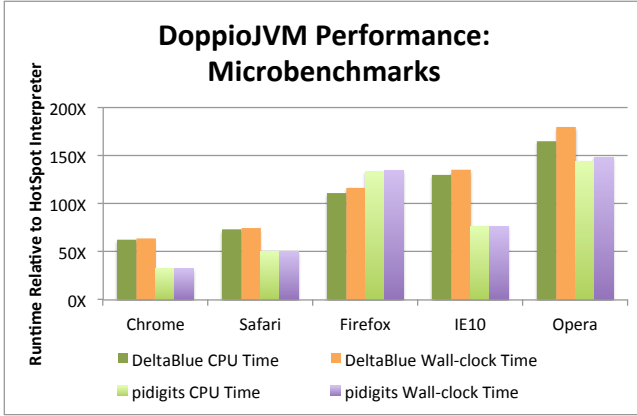
Figure 4. DOPPIOJVM performance on microbenchmarks relative to the HotSpot interpreter. CPU Time measures the amount of time that DOPPIOJVM actually spends executing the benchmark, while Wall-clock Time measures overall benchmark duration.
