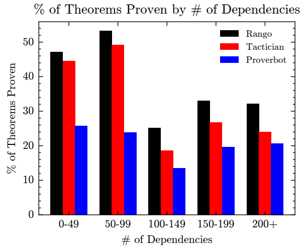
Fig. 6. Percentage of theorems proven by Rango, Tactician and Proverb by the number of dependencies of the current file to other files in the project.
