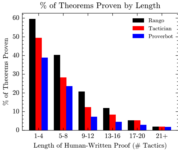
Fig. 5. Percentage of theorems proven by Rango, Tactician, and Proverb by the length of the human-written proof.
