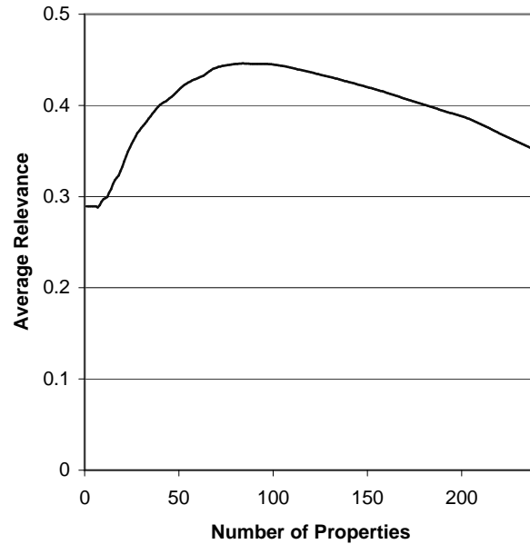
Figure 6-3: Relevance vs. set size averaged across all C program versions using the machine learner SVMfu. Beyond 250 properties, the relevance drops off approximately proportionally to the inverse of the set size. Property clusters, described in section 6.2, cause the flat part of the curve on the left side of the graph.
