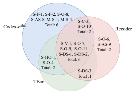
Fig. 7. The repair results of different APR tools
