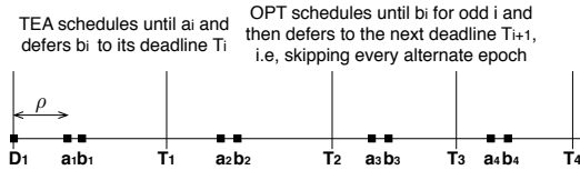
Figure 30: Illustration for showing that any TEA -style algorithm can be a factor 2 worse than optimal.
