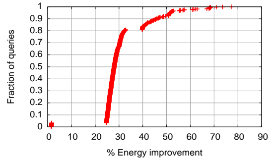
Figure 21: Web search: CDF of the energy improvement using TailEnder
