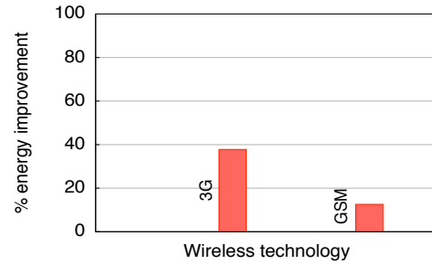
Figure 20: Web search: Average per query energy improvement using TailEnder for Web search over 3G and GSM
