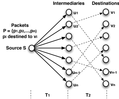
Figure 16: Theorem 1(a) construction: Solid arrows represent node meetings ALG known a priori while dotted arrows represent meetings ADV generates and reveals subsequently.
