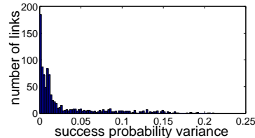
Figure 1: Histogram of the variance of the success probabilities of all links.
