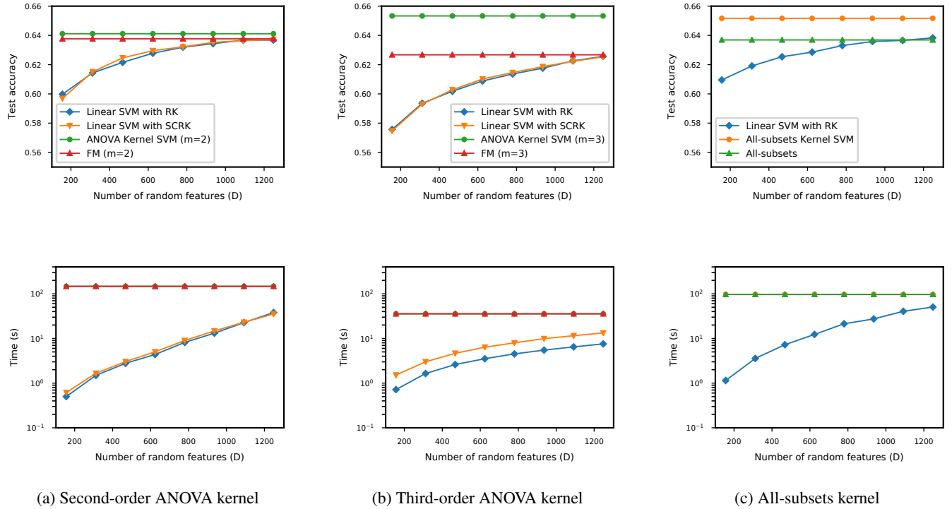
Figure 2: Test accuracies and times for linear SVM using RK feature map approximating (a) second-order ANOVA kernel, (b) third-order ANOVA kernel, and (c) all-subsets kernel and for two existing methods for Movielens 100K dataset. Upper graphs show test accuracies; lower ones show training and test times (time is shown in log scale).
