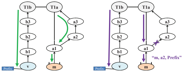
Figure 11: False loop prefix hijack.
