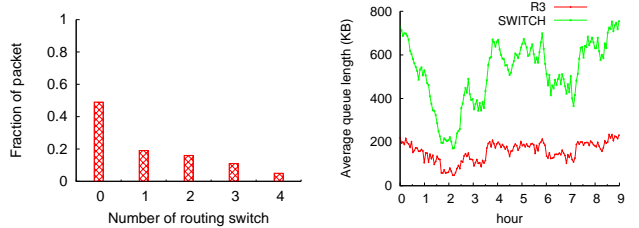
Figure 15: [Haggle] Analyzing SWITCH forwarding.
