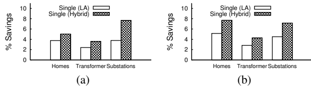
Figure 6: Savings from deploying hybrid storage technologies at a single-level for low and high cap-ex costs under long-term contract.
