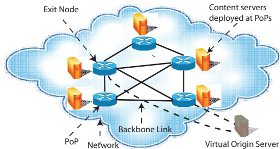
Figure 2: NCDN Architecture
