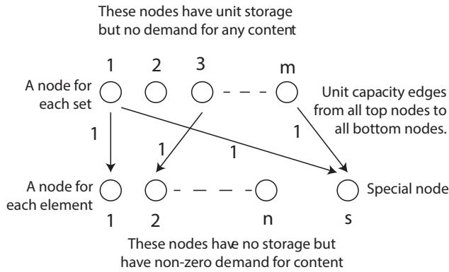
Figure 15: Reduction from SetCover to Opt-NCDN
