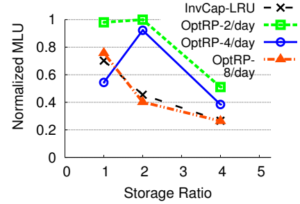
Figure 12: [Entertainment, US-ISP] OptRP does not outperform InvCap-LRU despite engineering 8 times a day.
