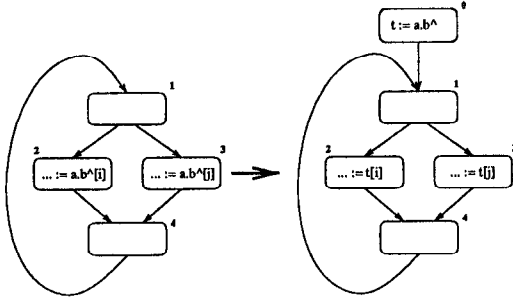
Figure 6: Eliminating Loop Invariant Memory Loads
