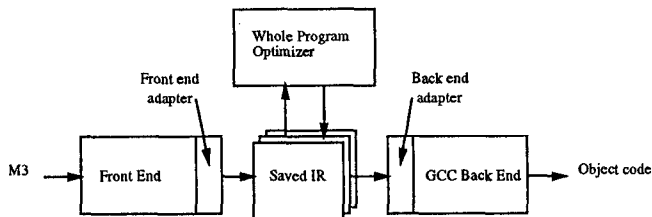
Figure 5: Compilation Framework
