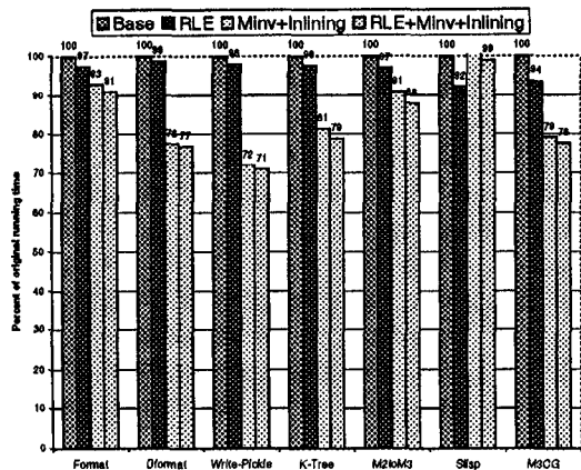
Figure 11: Cumulative Impact of Optimizations
