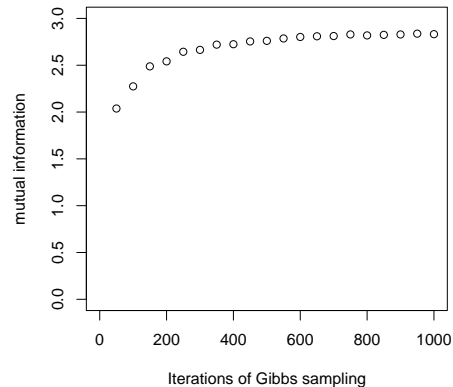
Mutual Information between Author and Topic
