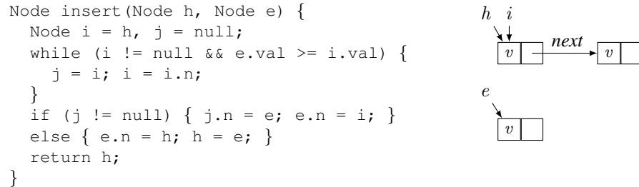
Fig. 3. Sample counterexample generated for a buggy version of insert . Here, the loop invariant required that \forall \alpha : (h \langle next^* \rangle \alpha \wedge \neg i \langle next^* \rangle \alpha) \rightarrow \alpha <_{val} e (where <_{val} is an ordering on nodes according to their values), but the loop will execute one more time, violating this.
