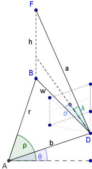
Fig. 5. The geometry of the bisight tilt. \sigma represents the angle of tilt, while \lambda represents the additional vertical angle displacement of the ray to the feature F. \psi (not shown) is the sum of \sigma and \lambda .
