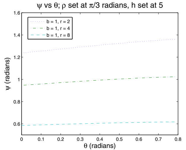
Fig. 6. Graph showing approximately linear relationship between \psi and the bisight mount's pan angle ( \theta ) (see text).
