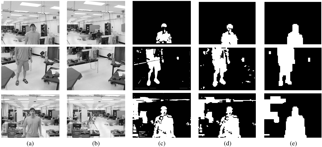
Fig. 7. Three examples: (a) input image with foreground object, (b) closest background image from stored set of persistent background images, (c) image differencing and threshold after global alignment, (d) image differencing after local matching, (e) classification of foreground/background by discriminative Markov random field.
