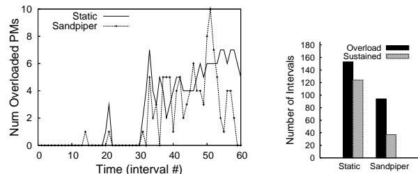
Figure 9: Sandpiper eliminates all hotspots and reduces the number of intervals experiencing sustained overload by 61% .
