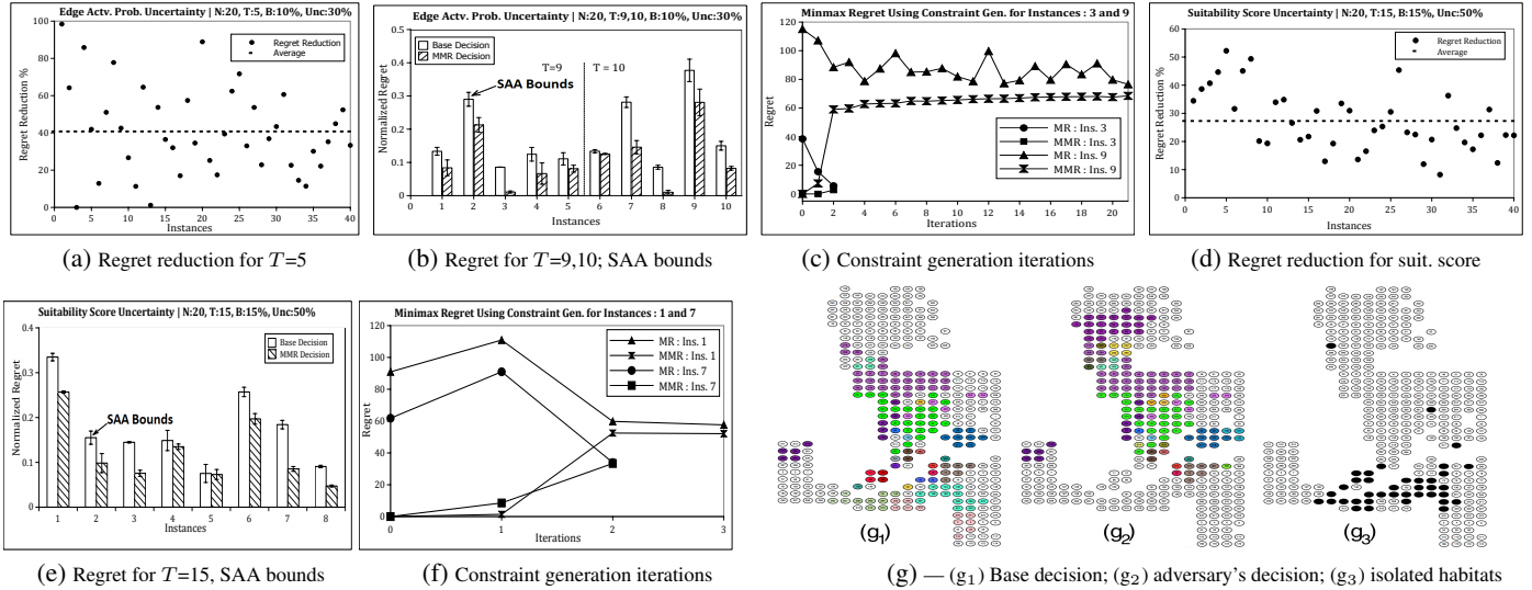
Figure 2: Regret analysis for edge activation probability and suitability score uncertainty. Figure (g) best viewed electronically
