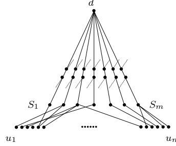
Figure 3: Reduction from set cover.
