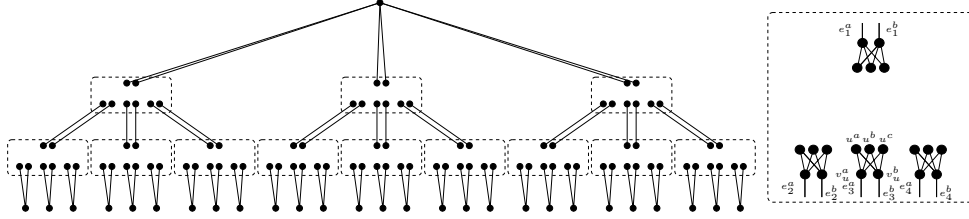
Figure 1: Reduction from LONGESTPATH to MINHOP 2 (undirected).
