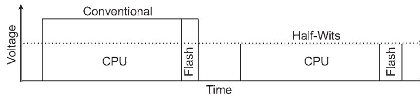
Fig. 1. Operating at a lower voltage and tolerating errors instead of the conventional case of choosing the highest minimum voltage requirement may help decrease energy consumption. Considering that Power \propto voltage^2 , decreasing voltage decreases the power consumption quadratically.
