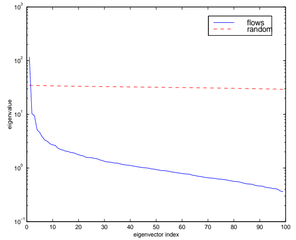
Figure 3: The eigenvalues of the color flow covariance matrix. The rapid drop off in magnitude indicates that a small number of eigenflows can be used to represent most of the variance in the distribution of flows.
