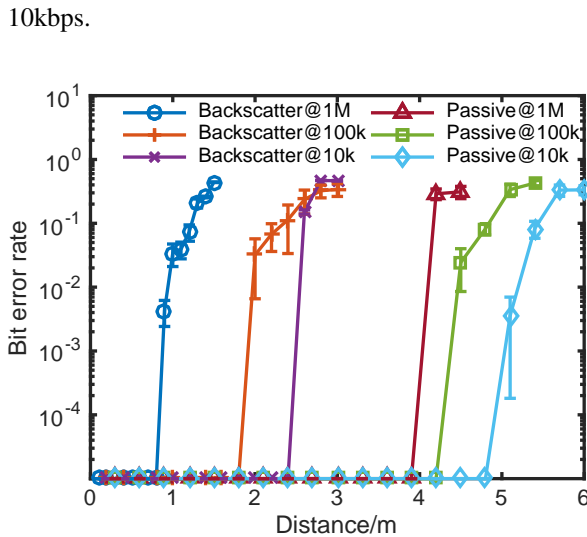
Figure 13: Bit error rate over distance for backscatter and passive receiver modes at different bitrates.
