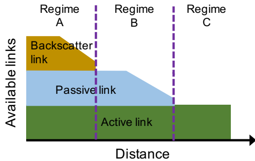
Figure 8: Three operating regimes of Braidio
