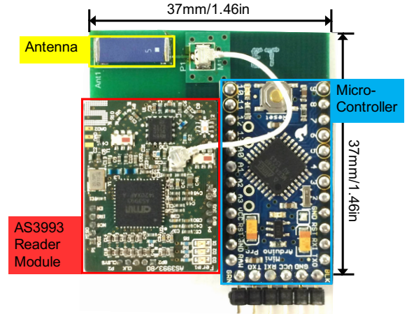
Figure 11: AS3993 reader test board
